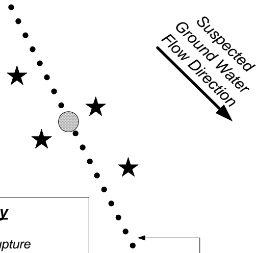
Figure 3-1f. Generalized high-volume pipeline release with limited or no contaminated surface soils. The immediate vicinity of the point of pipeline rupture would be considered the source area. A minimum of four borings/monitoring wells would be placed around the point of release, including upgradient, downgradient, and both cross-gradient locations. This release would be ineligible for Title 200 reimbursement.
