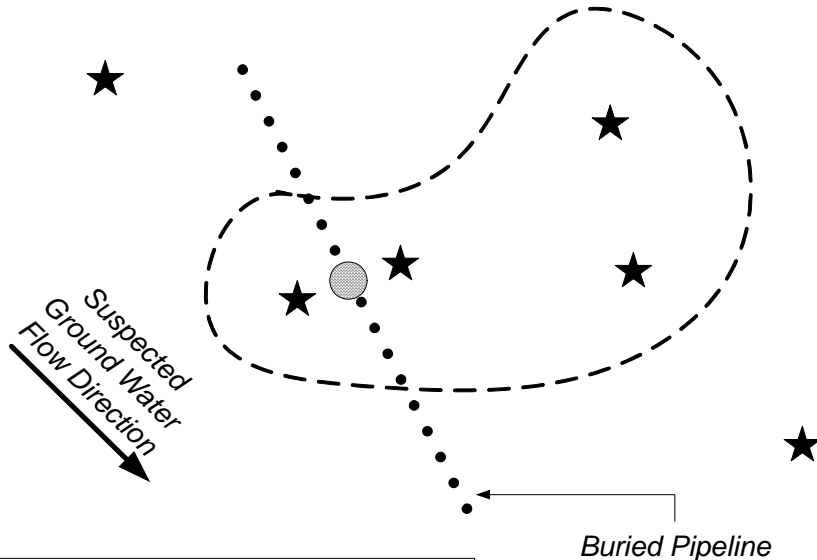
Figure 3-1e. Generalized high-volume pipeline "blowout" resulting in large volume petroleum release with an area of contaminated surface soils. This release would be ineligible for Title 200 reimbursement. The actual number of source area borings/monitoring wells (denoted by the stars within the spill area) will vary based on the size of the spill area and consultation with the Department. For such a surface release, low-lying areas where product may pool are likely candidates for boring placement. Upgradient and downgradient monitoring wells should be included.
