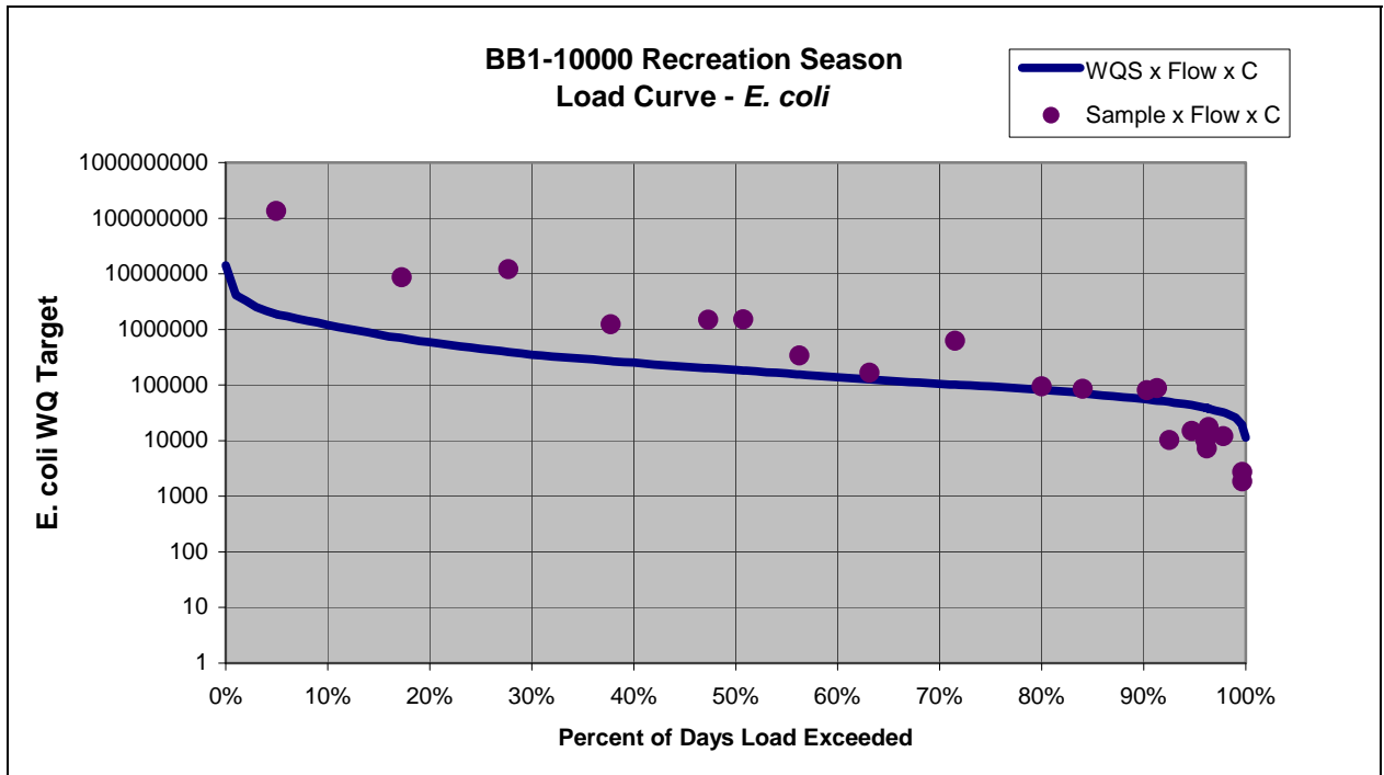
Figure 2.3.1a. Load Curve for BB1-10000
